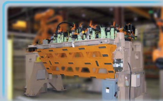
Trunnion (automotive sector)
